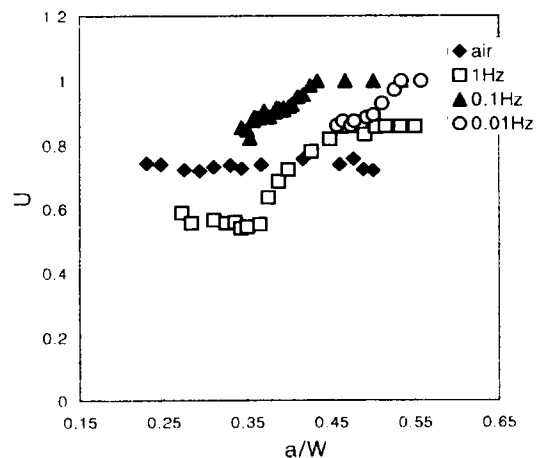
Fig. 7 Relationship between U and a/W
