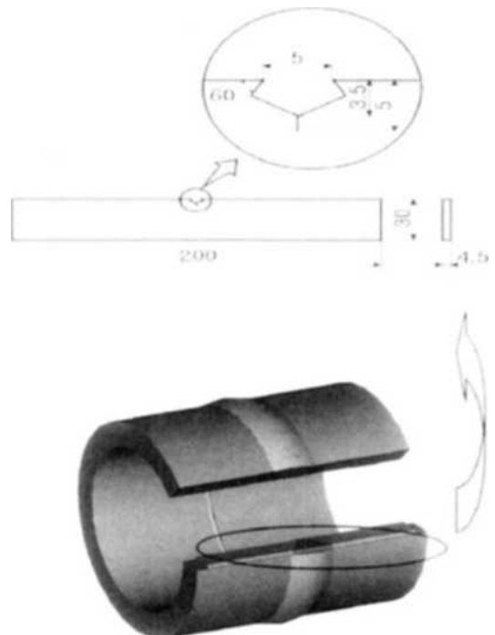
Fig. 1 Configuration and position of specimen
