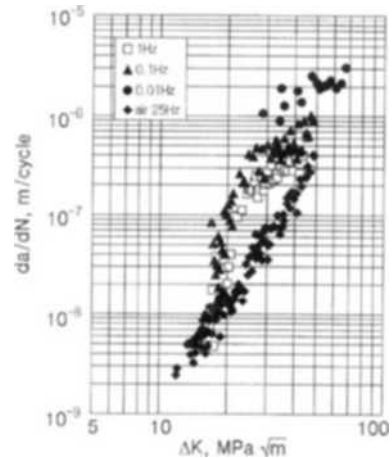
Fig. 3 Corrosion fatigue characteristic curves
