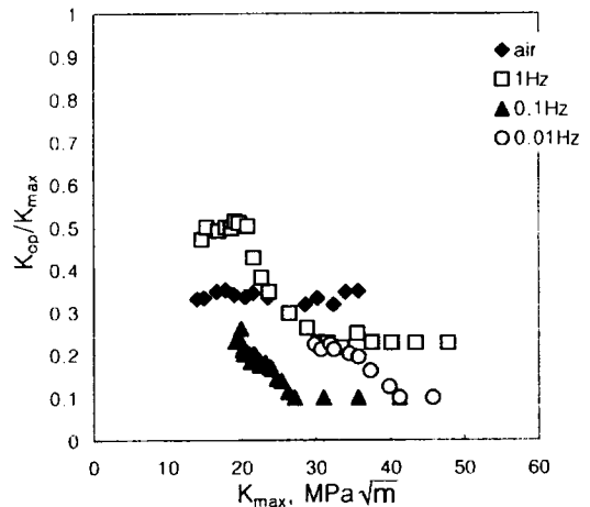
Fig. 6 Relationship between K_{op}/K_{max} and K_{max}
