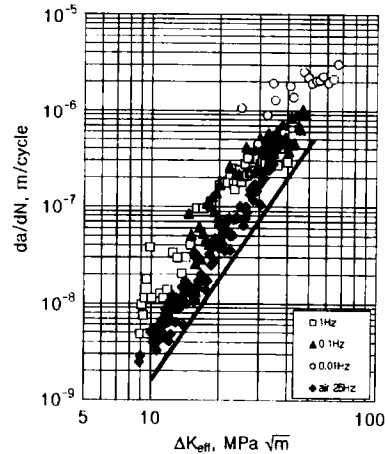
Fig. 8 Representation of corrosion fatigue characteristic curves of Fig. 3 using \Delta K_{\text{eff}}
